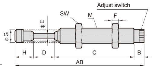
帶有塑膠頭彈簧 Have head and spring
