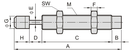
帶有塑膠頭 Have head
