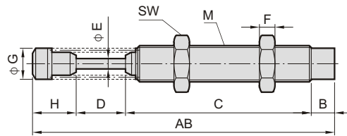
帶有塑膠頭彈簧 Have head and spring
